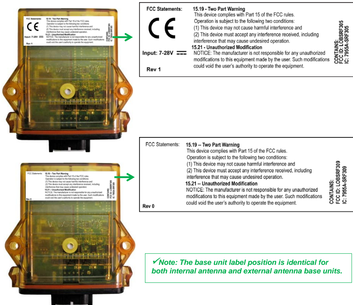
Figure 8. Agency Identification Label Locations
