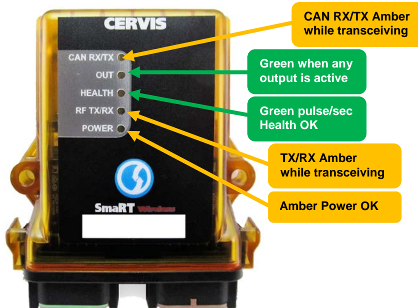
Figure 1. BU-xH6R LEDs
