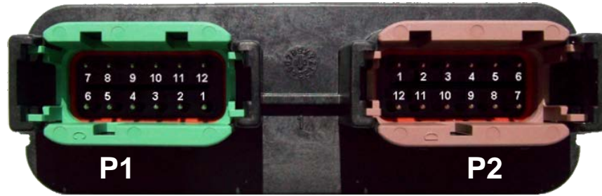
Figure 5. Dual Connectors/Pin Numbers (enhanced)
