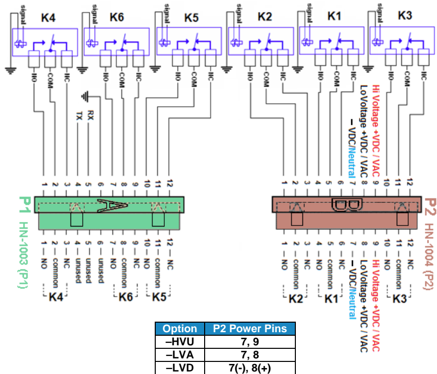
Figure 6. P1 and P2 Field Wiring Layout
